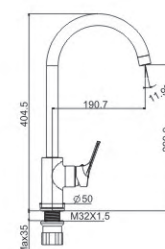
M54964-374C Vertical kitchen faucet
