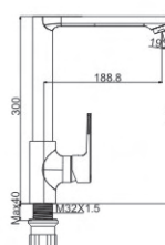
M54441-200C Vertical kitchen faucet
