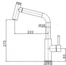
M53567-006C-548 Pull out spray kitchen faucet
