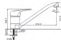
M51004-502C-S100 Vertical kitchen faucet
