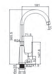
M54571-236C Vertical kitchen faucet
