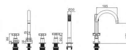
M82686-991C-C589 Bath faucet
