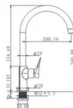
M54994-8021CH Vertical kitchen faucet
