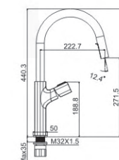
M53783-833C-S623 Pull out spray kitchen faucet
