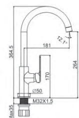
M54795-845C Vertical kitchen faucet
