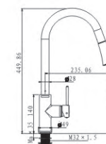
M53836Q Pull out spray kitchen faucet
