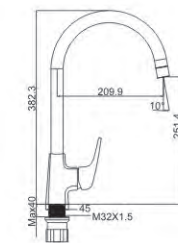
M54386-161C-S259 Vertical kitchen faucet
