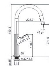
M53783-833Q-S623 Pull out spray kitchen faucet
