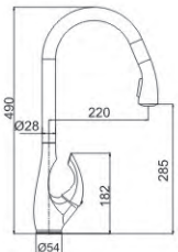
M53880-377C Pull out spray kitchen faucet
