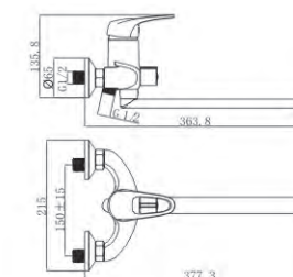
M33027-502C-S023 Wall bath faucet
