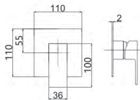
M63545-819C Concealed shower faucet
