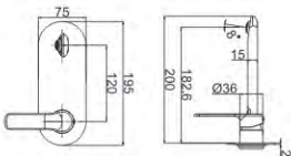
M61795-845C Concealed basin faucet
