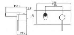
M61883-8006C Wall basin faucet
