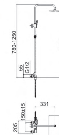
M92787-842C Shower set
