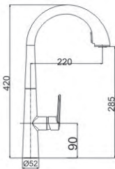
M53892-355C Pull out spray kitchen faucet
