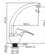
M54004-530C-C258 Vertical kitchen faucet
