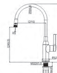
MZ54860-345C-S07682 Kitchen faucet with silicone spout two functions Zinc faucet body with brass core
