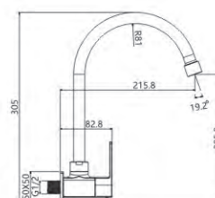
M02021-821C Wall kitchen faucet
