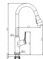
M53826Q Pull out spray kitchen faucet
