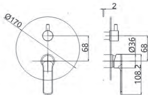
M64795-845C Concealed shower faucet
