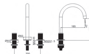
M81730-998C-C589 Basin faucet
