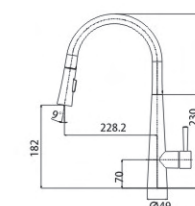
M53576-232Q-553 Pull out spray kitchen faucet
