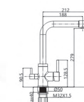
M54510-207C Kitchen faucet with drinking water
