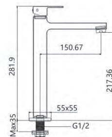
M03013-809C Basin faucet
