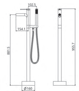
M93883-8006C Freestanding faucet
