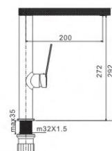
M54634-828HRG Vertical kitchen faucet
