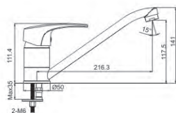
M51004-530C-S100 Vertical kitchen faucet
