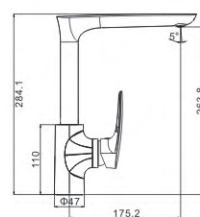
M54689-292C Vertical kitchen faucet
