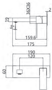
M62545-819C Concealed basin faucet
