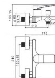
M31920-8013C Bath faucet
