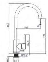
MZ54804-006C-S07545 Kitchen faucet Zinc faucet body with brass core
