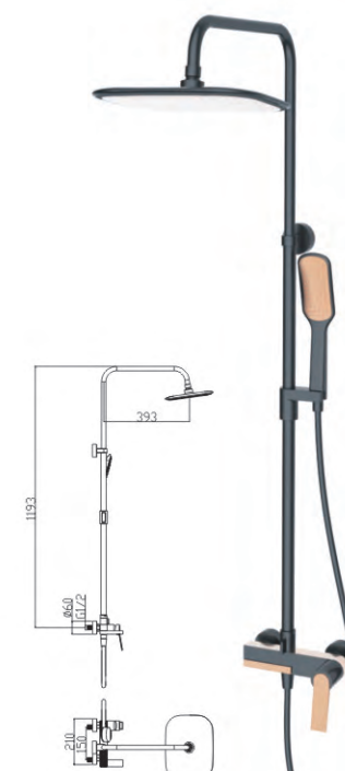
M92634-268HRG Shower set
