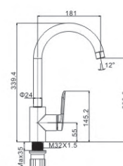
M54570-235C Vertical kitchen faucet
