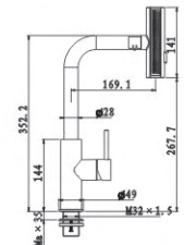
M53567-232C-548-P25266 Pull out spray kitchen faucet
