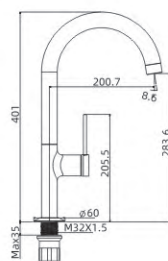
M54883-8006C Vertical kitchen faucet
