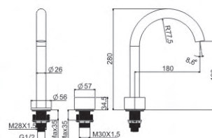
M81929C Basin faucet
