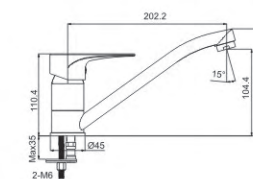
M51034-118C-S080 Vertical kitchen faucet
