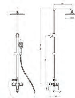
M92571-236C Shower set
