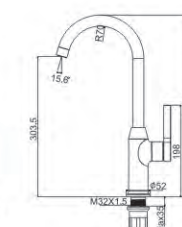
MZ54860-345C-S07680 Kitchen faucet Zinc faucet body with brass core
