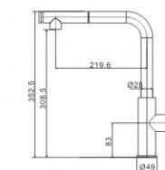
M53567-232LSJ-547 Pull out spray kitchen faucet
