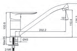
M51034-120C-S080 Vertical kitchen faucet
