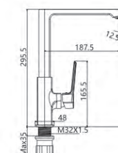
M54835-849C Vertical kitchen faucet
