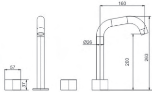
M82928Q Basin faucet
