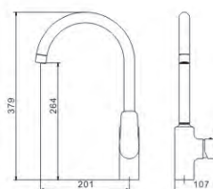
M54776-317C Vertical kitchen faucet
