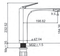
MI288I-353LG Basin faucet
