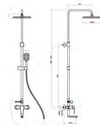
M92571-236HRG Shower set
