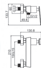
M41797-847LSJ Shower faucet
