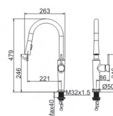
M53805-329Q-C627 Pull out spray kitchen faucet
