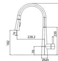
M53576-232C-553 Pull out spray kitchen faucet
