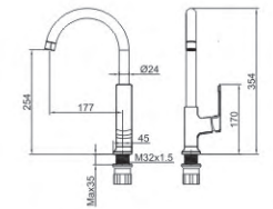
M54785-323Q Vertical kitchen faucet
