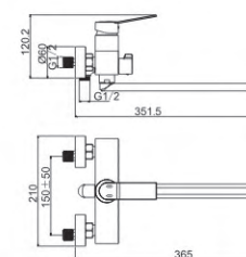
M33634-268HRG Wall bath faucet
