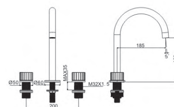
M81715-997C-C589 Basin faucet
