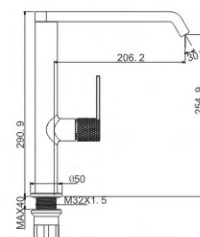
M54633-827LSJ Vertical kitchen faucet
