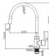
M54949-006C-S07679 Kitchen faucet with silicone spout one function Brass body
