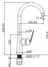
M5488I-353LG Vertical kitchen faucet
