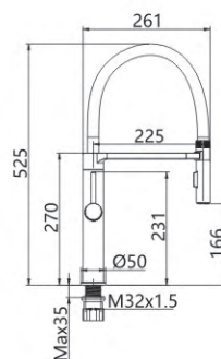
M5480I-817C Pull out spray kitchen faucet
