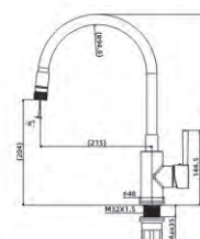
MZ54804-006C-S07683 Kitchen faucet with silicone spout two functions Zinc faucet body with brass core
