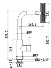
M53783-833Q-548-P25266 Pull out spray kitchen faucet
