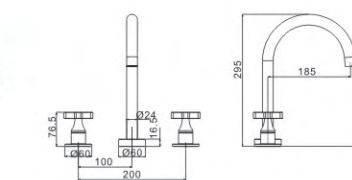
M81686-991H-C589 Basin faucet
