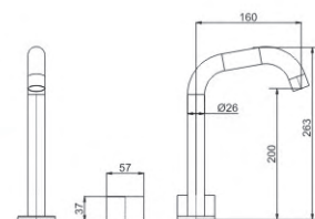
M81928Q Basin faucet
