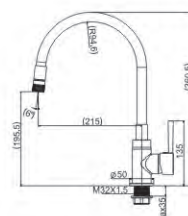
M54949-006C-S07682 Kitchen faucet with silicone spout two functions Brass body
