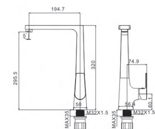
M54612-259C Vertical kitchen faucet
