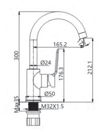
M54950-368C Vertical kitchen faucet
