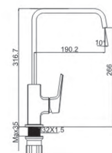
M54387-162C Vertical kitchen faucet
