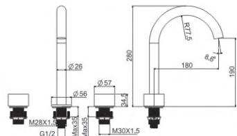
M82929Q Basin faucet
