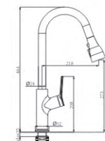
M53826C Pull out spray kitchen faucet
