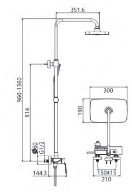
M92950-368C Shower Set
