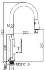
M53531-216Q Pull out spray kitchen faucet
