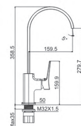
M54668-830Q Vertical kitchen faucet
