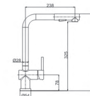
M53879-367C Pull out spray kitchen faucet
