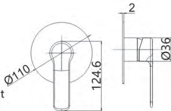
M63795-845C Concealed shower faucet
