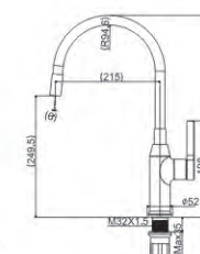
MZ54860-345C-S07679 Kitchen faucet with silicone spout one function Zinc faucet body with brass core
