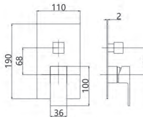
M64545-819C Concealed shower faucet
