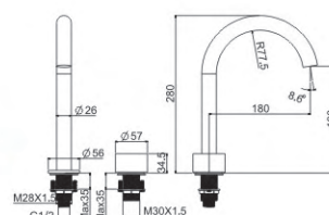
M81929LSJ Basin faucet
