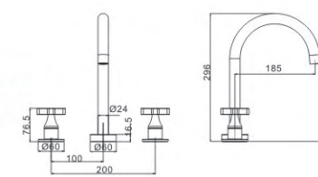
M81686-991C-C589 Bath faucet
