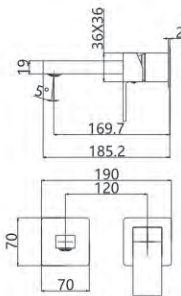
M61545-819C Concealed basin faucet
