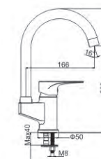
M54323-118C-C140 Vertical kitchen faucet
