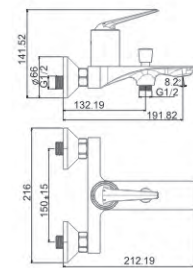
M3188I-353LG Bath faucet
