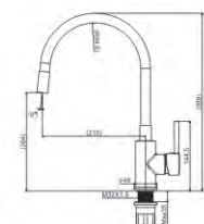
MZ54804-006C-S07626 Kitchen faucet with silicone spout one function Zinc faucet body with brass core
