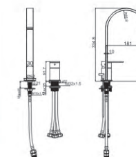
M81508-206C-C555 Basin faucet
