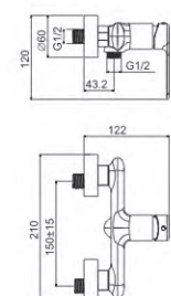
M41795-845C Shower faucet
