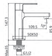
M02019-821C Basin faucet
