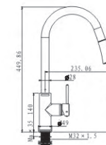
M53836C Pull out spray kitchen faucet
