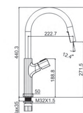
M53783-833HRG-S623 Pull out spray kitchen faucet
