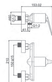
M4188I-353LG Shower faucet
