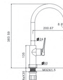
M54920-8013C Vertical kitchen faucet
