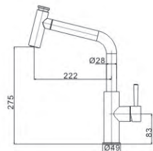
M53567-006H-548 Pull out spray kitchen faucet
