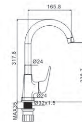
M54386-161C-C140 Vertical kitchen faucet
