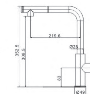
M53567-232H-547 Pull out spray kitchen faucet
