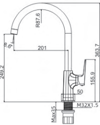
M54681-H275C Vertical kitchen faucet
