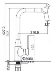
M53536-219C Pull out spray kitchen faucet
