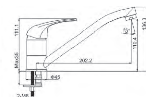
M51034-010C Vertical kitchen faucet
