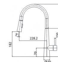
M53576-232H-533 Pull out spray kitchen faucet
