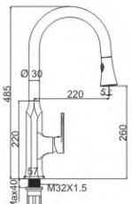
M53531-216NB Pull out spray kitchen faucet
