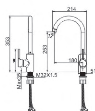
M54786-325CH Vertical kitchen faucet
