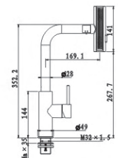
M53567-232H-548-P25266 Pull out spray kitchen faucet
