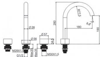
M82929C Basin faucet
