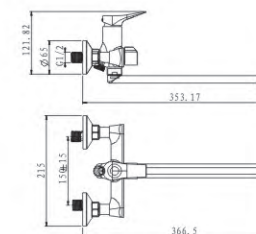
M33994-8021CH Wall bath faucet
