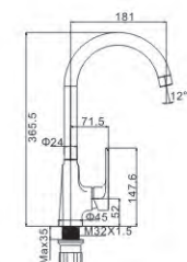
M54571-236HRG Vertical kitchen faucet
